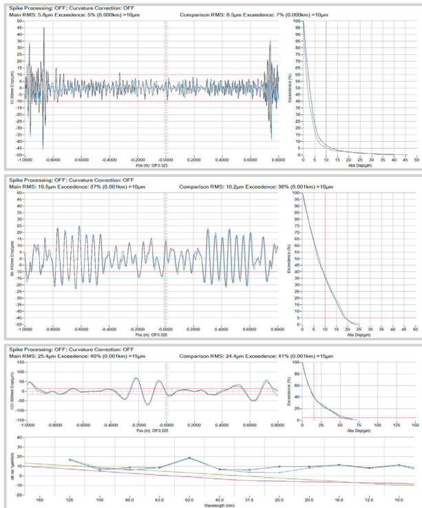
Typical calibration curves: CAT and CMM measurements of a 1.8m section of a calibration beam.
